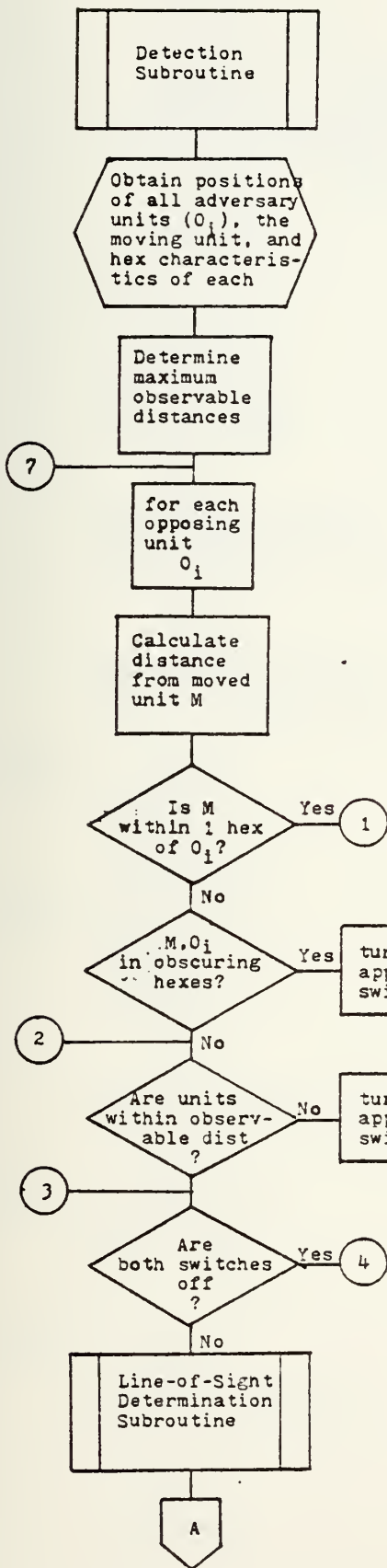
FIGURE V.10 FLOWCHART OF DETECTION SUBROUTINE
